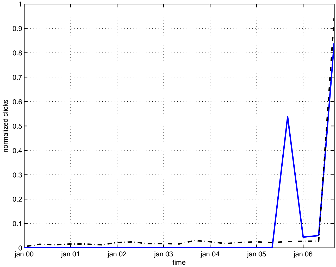
relativistic effect
