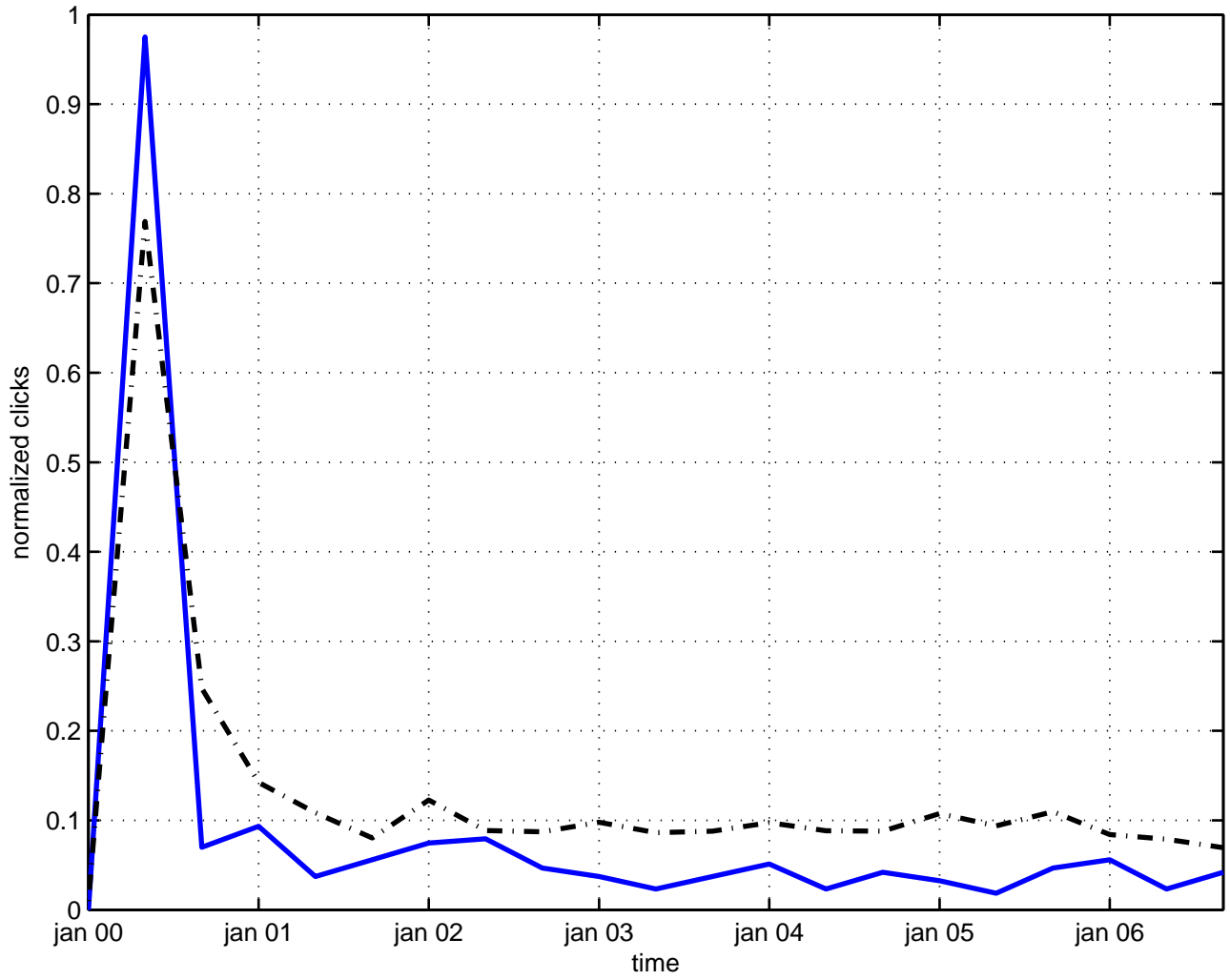
regularization potential
