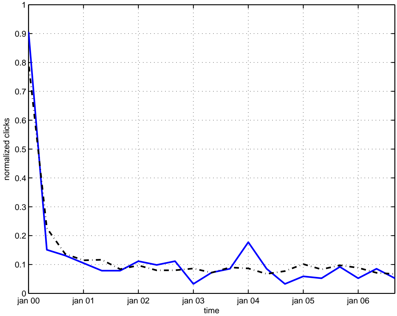
regularization partition function
