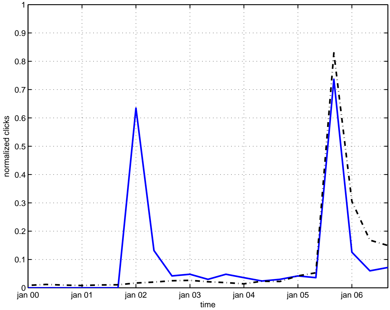
regularization operator
