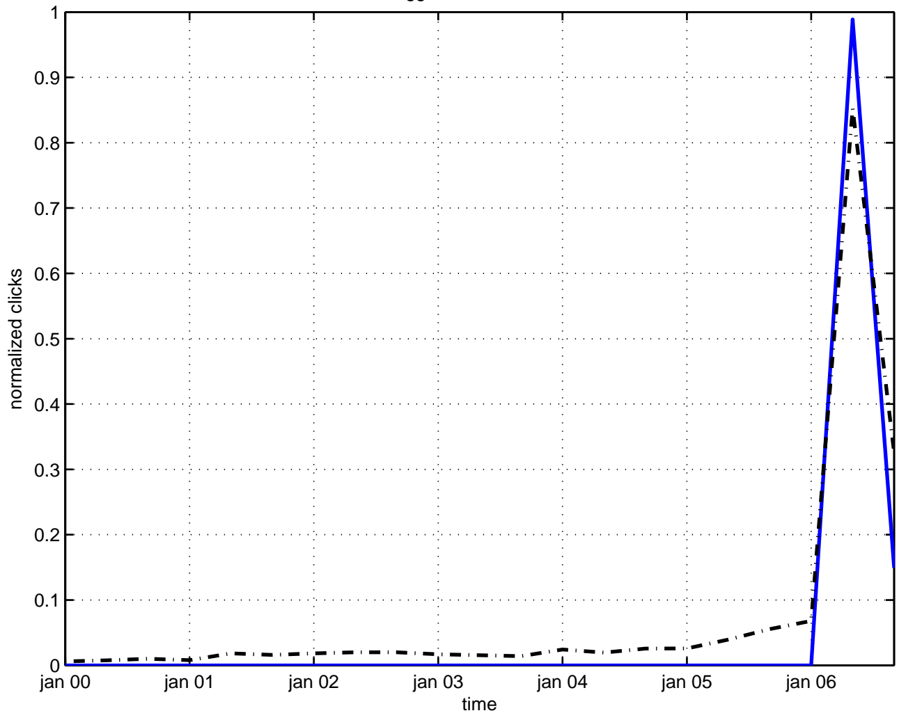
regge random surface
