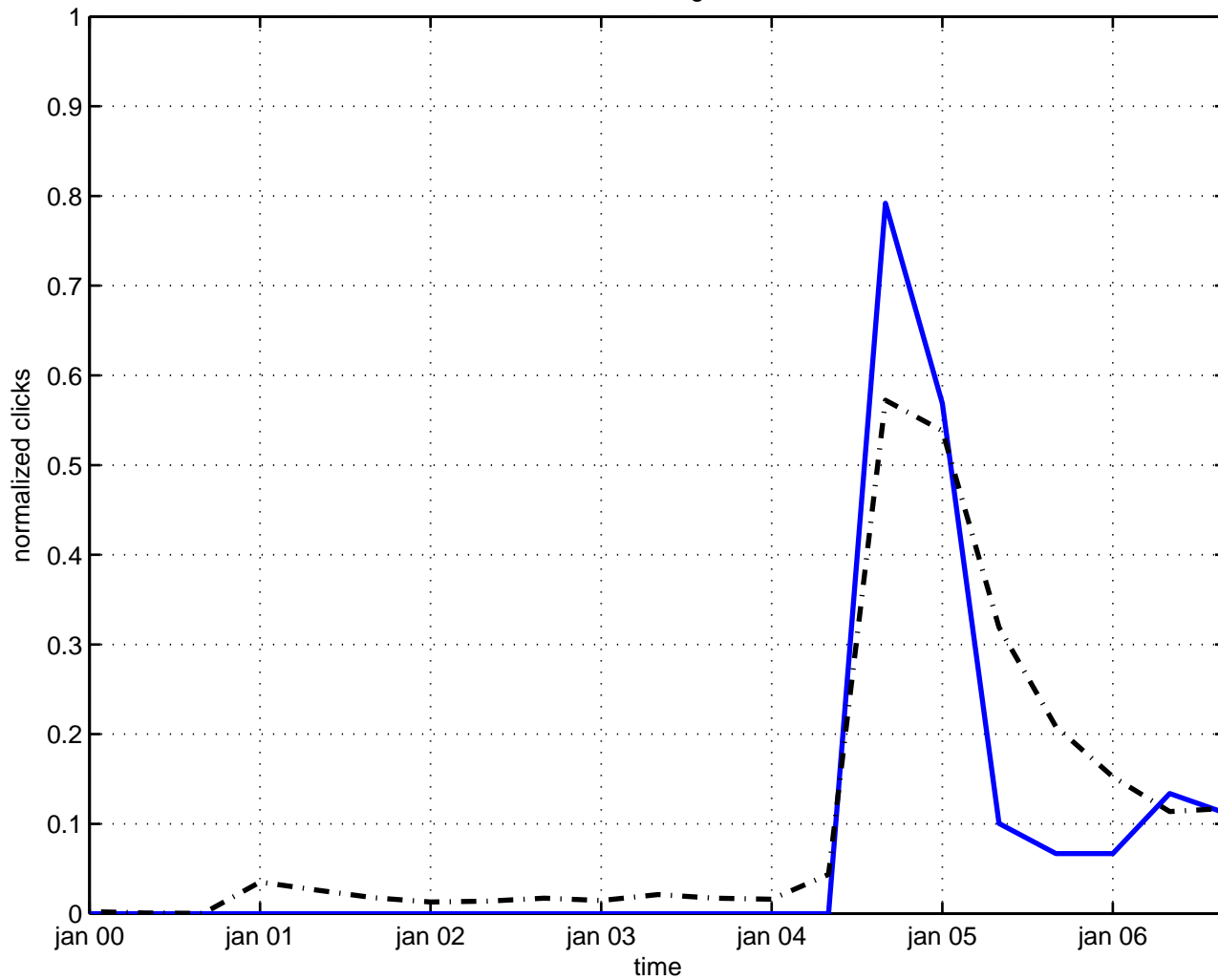
reflection algebra
