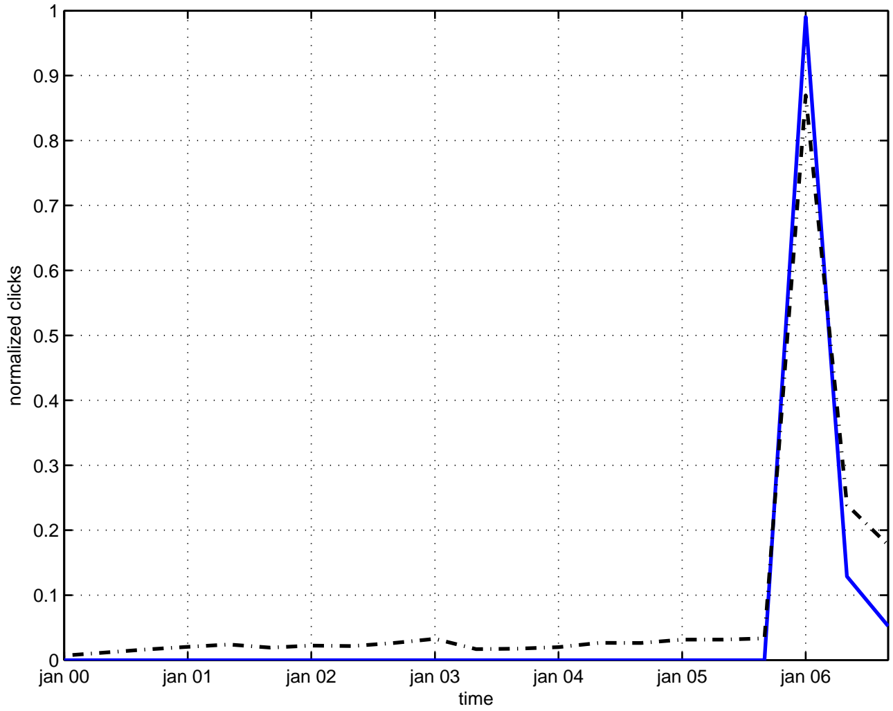
recoil black hole
