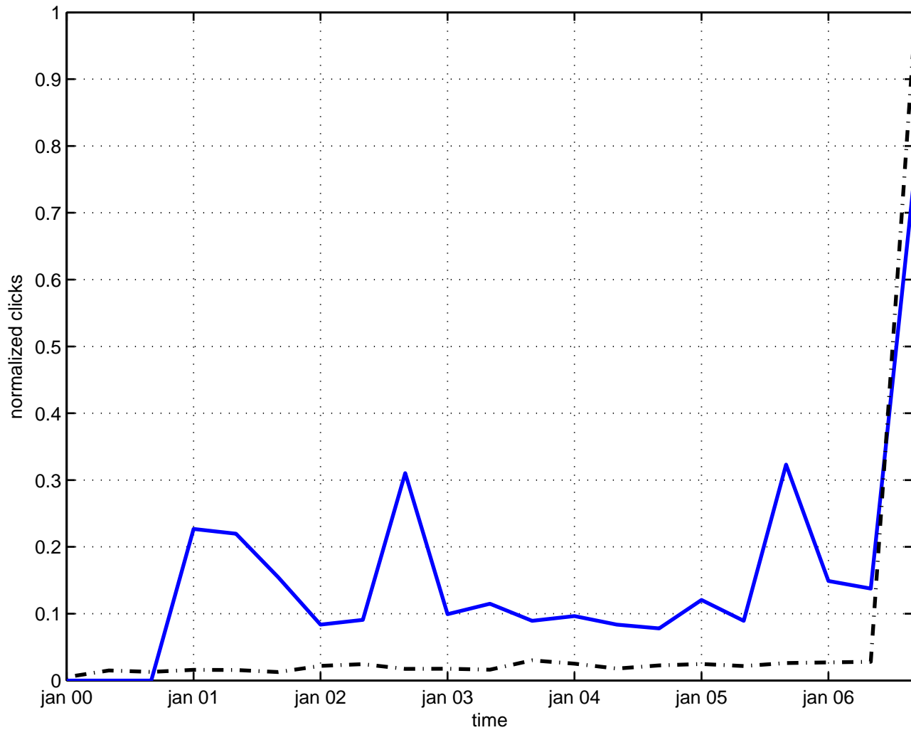
rational transformation
