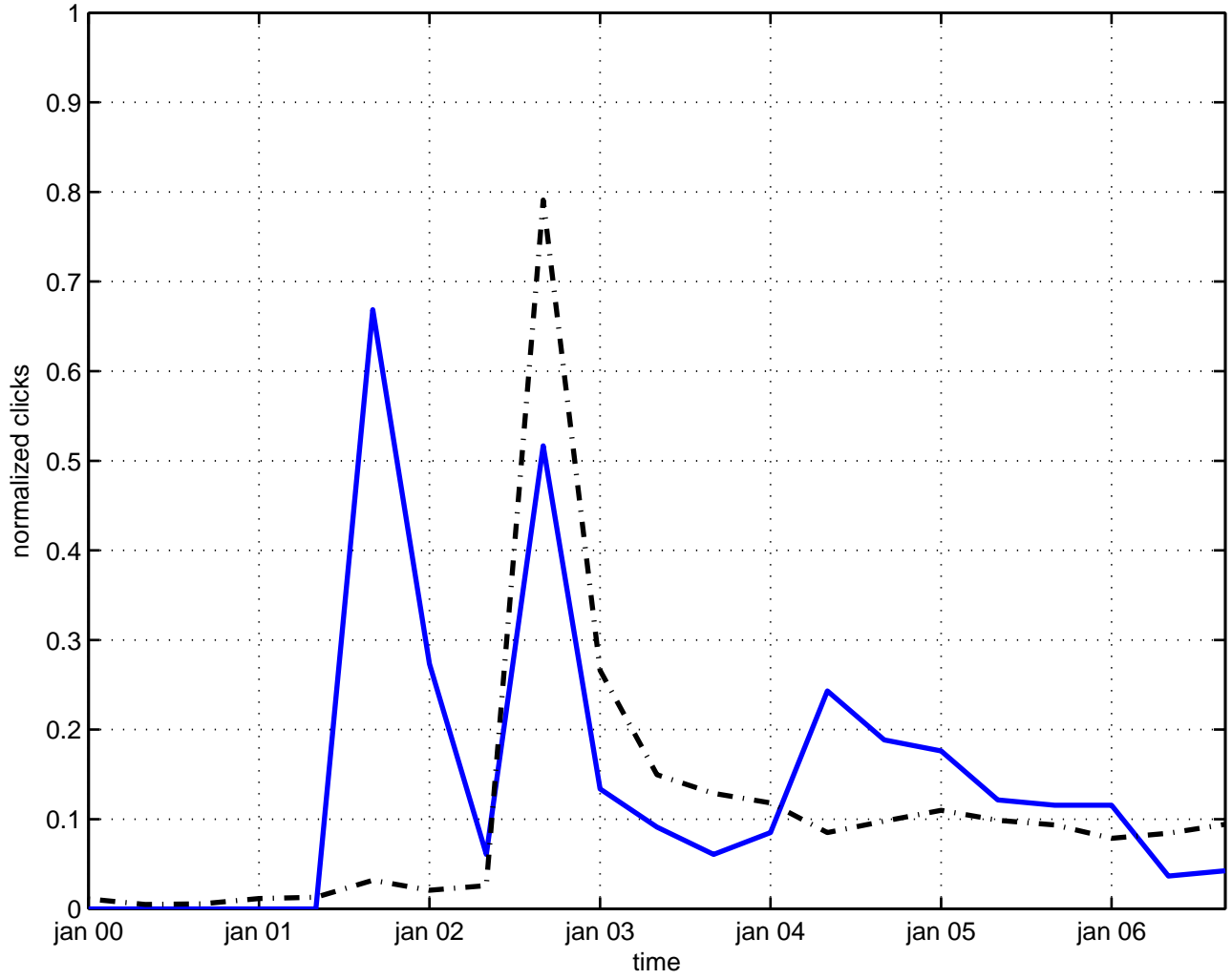
rational correlation function
