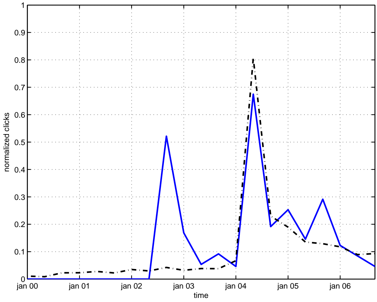
random statistical mechanics
