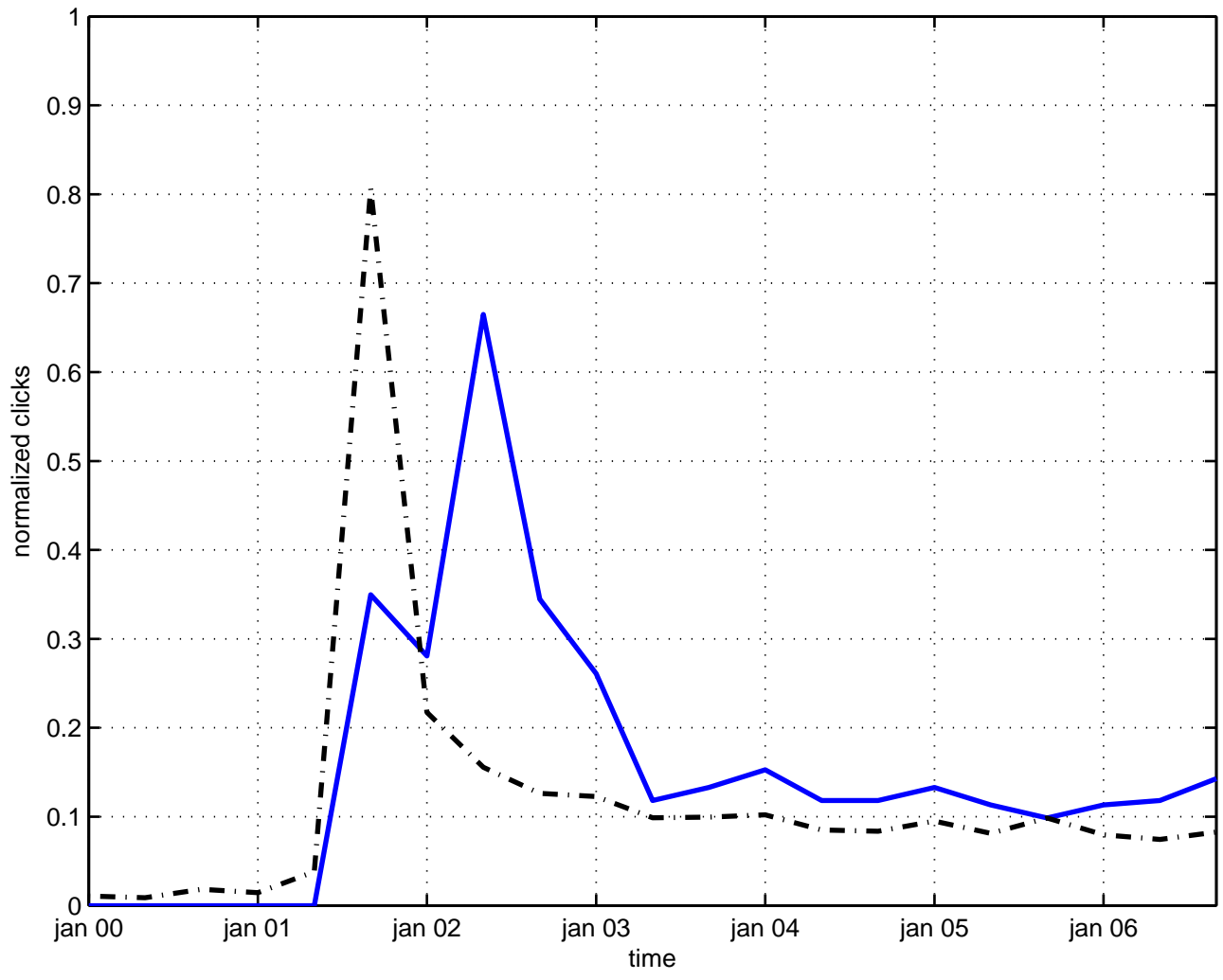
random field
