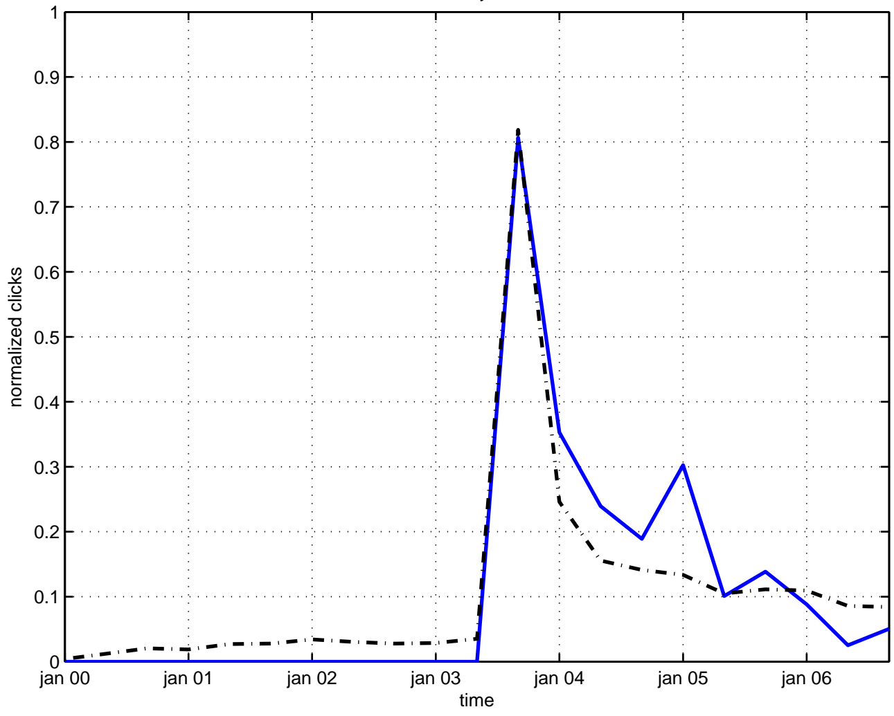
radiative decay bound state
