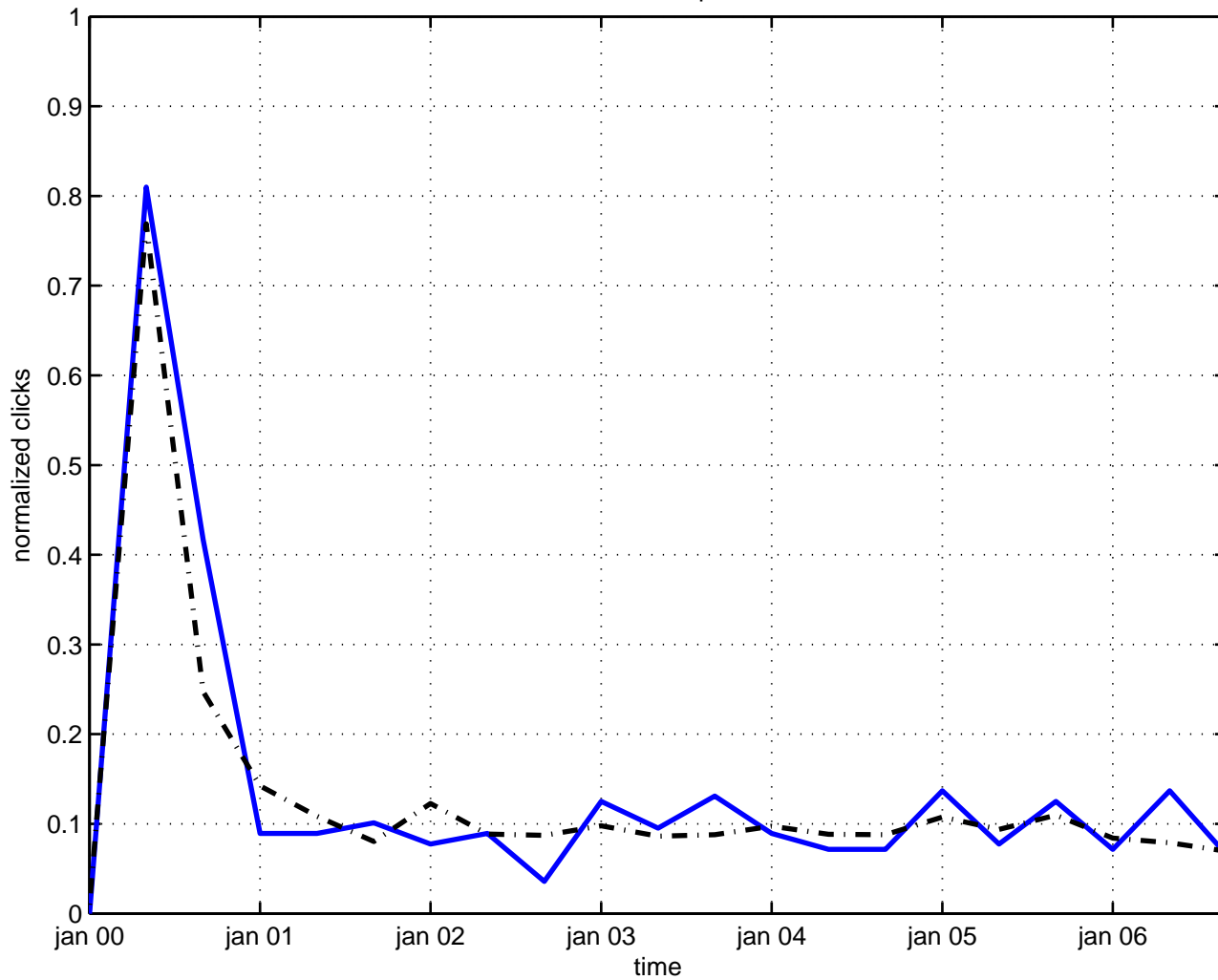
rademacher expansion
