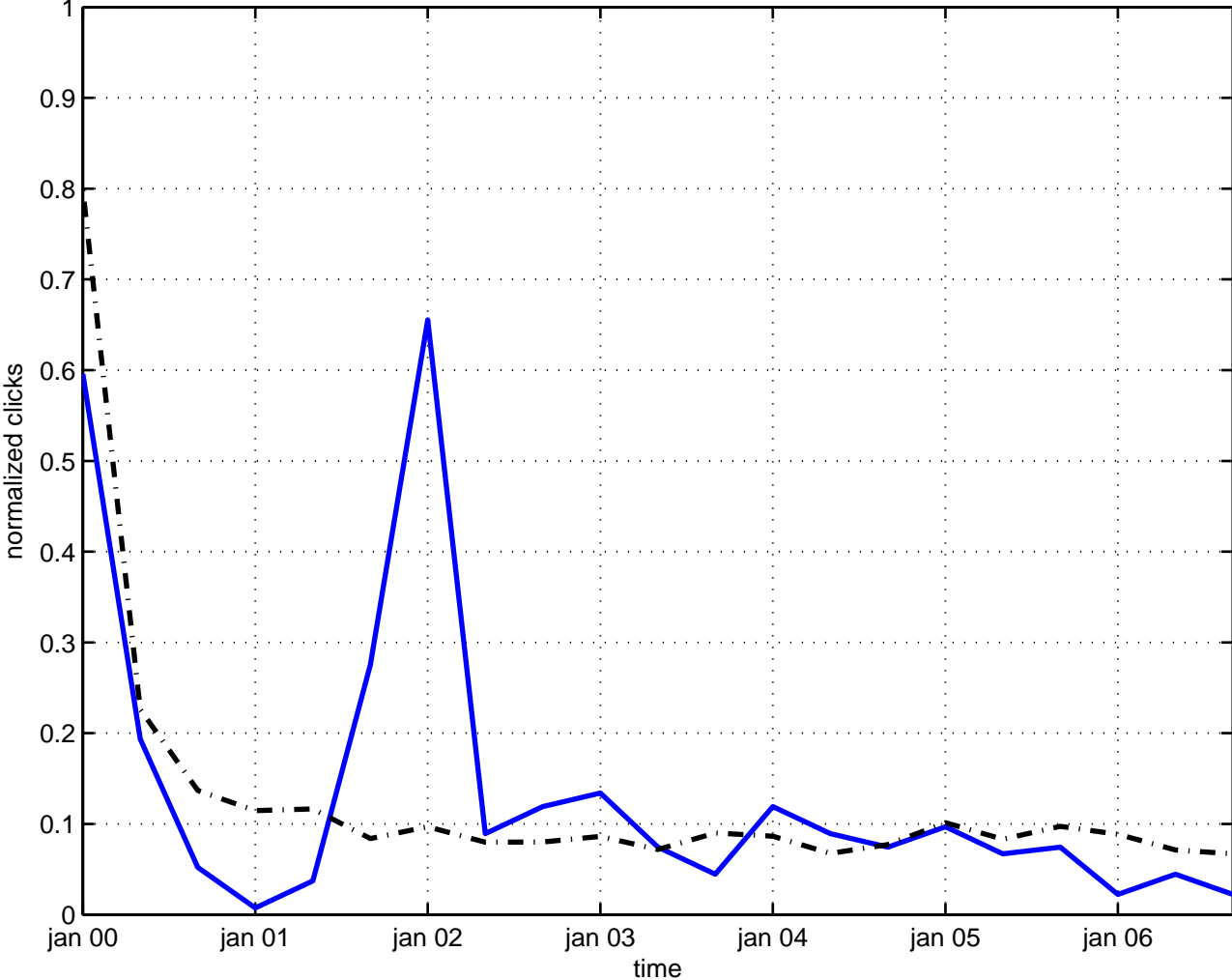
r-matrix yang-baxter equation
