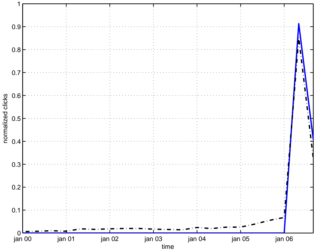
r(1) x s(3) space-time
