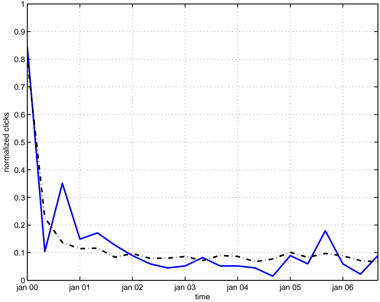
r(1) x s(1) space-time
