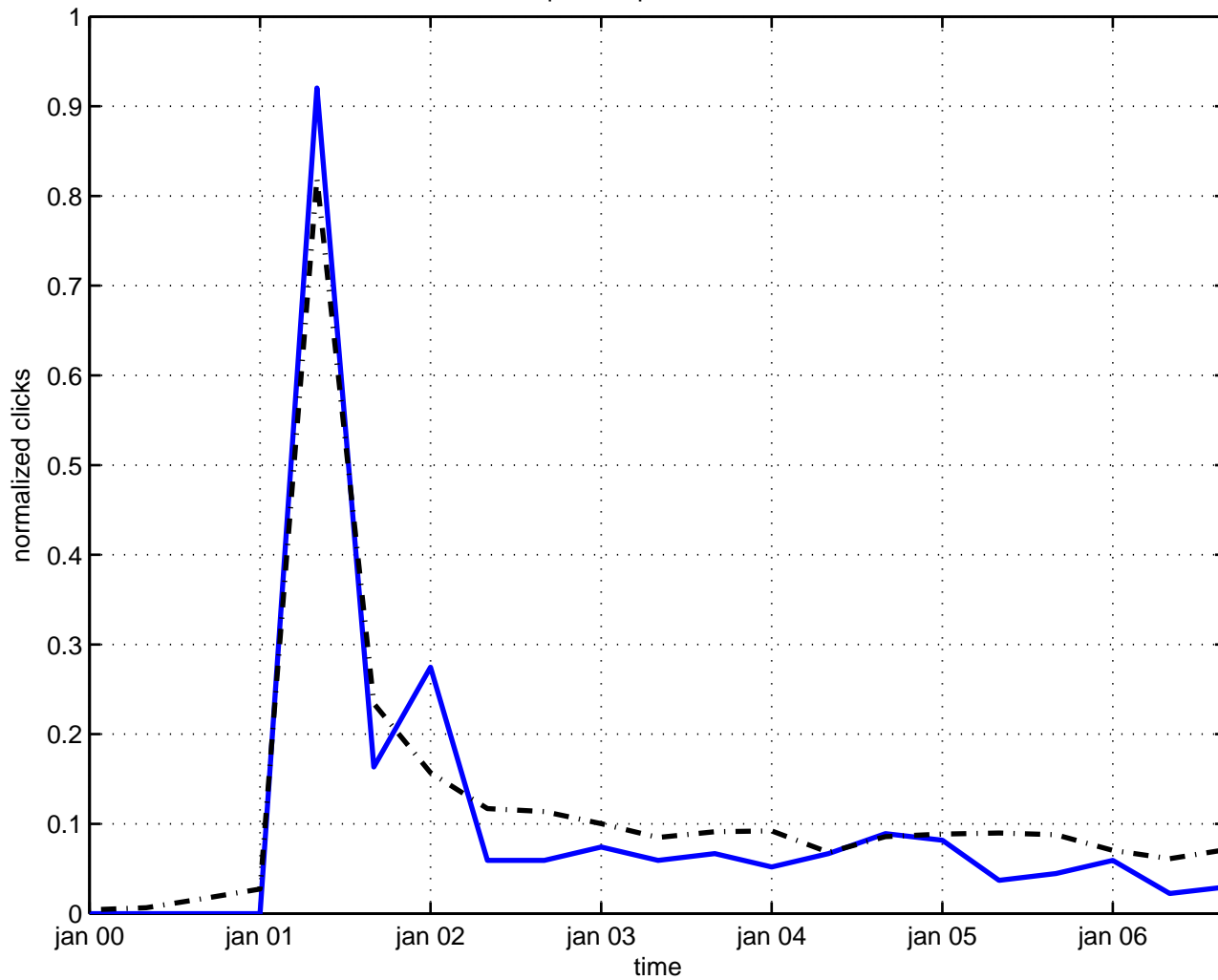
quiver representation
