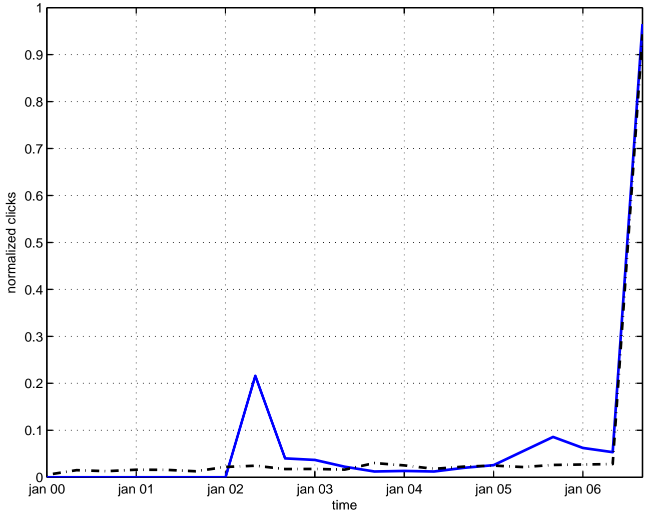
quiver quantum mechanics
