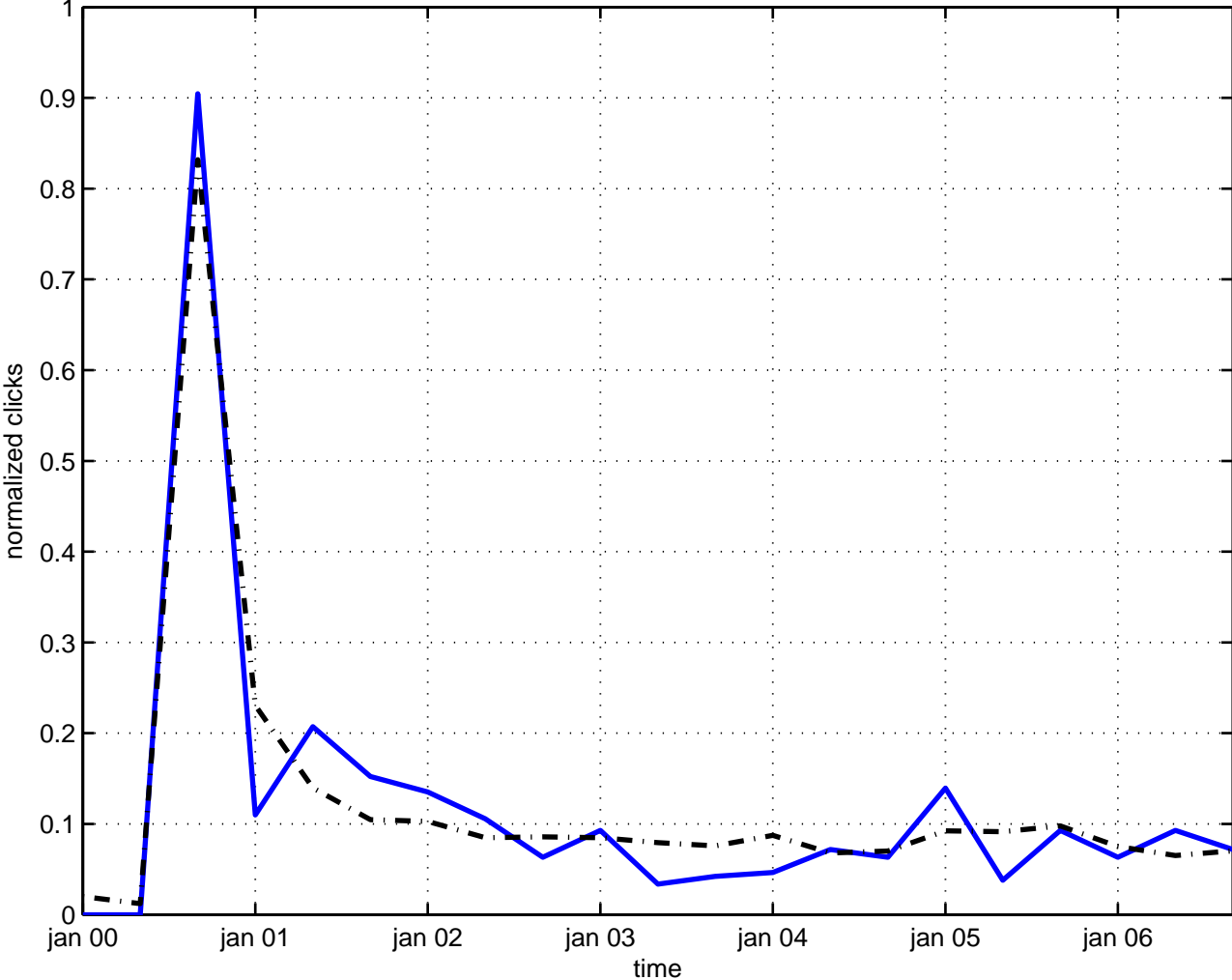
quiver group theory
