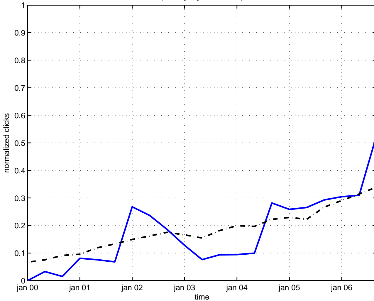
quiver gauge field theory
