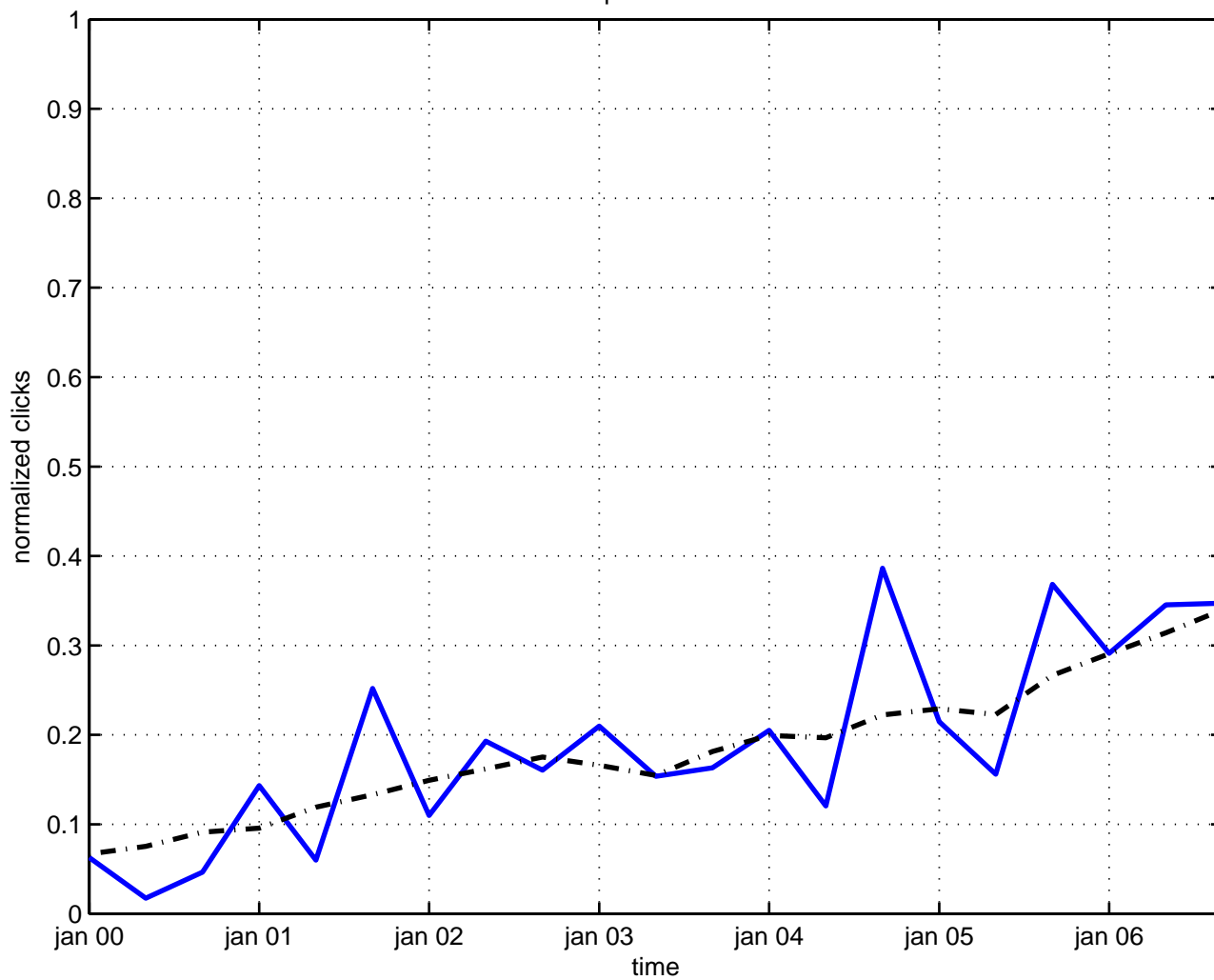
quaternion
