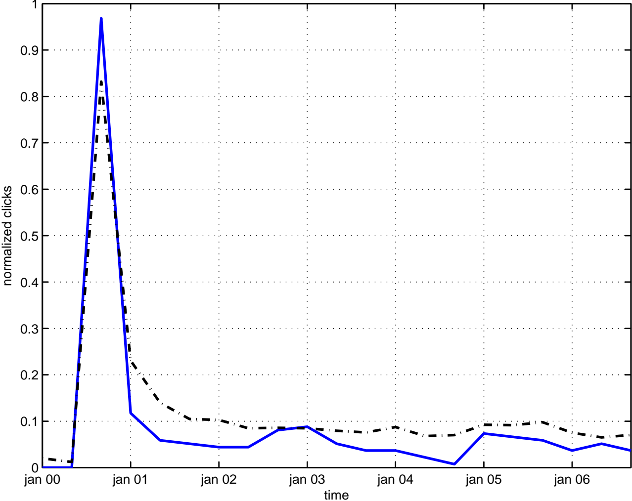
quasiparticle boson
