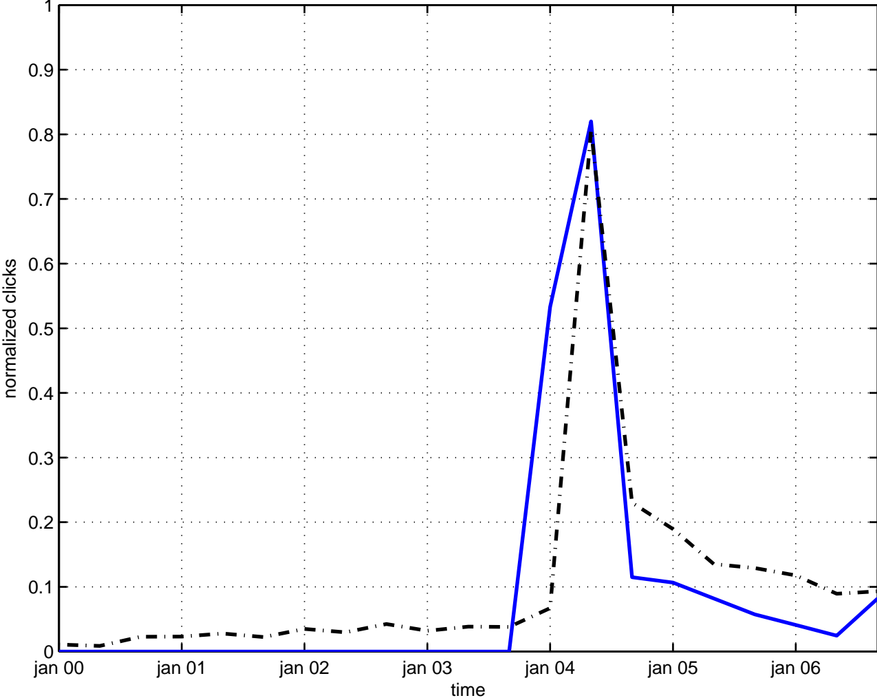
quantum mechanics supersymmetry
