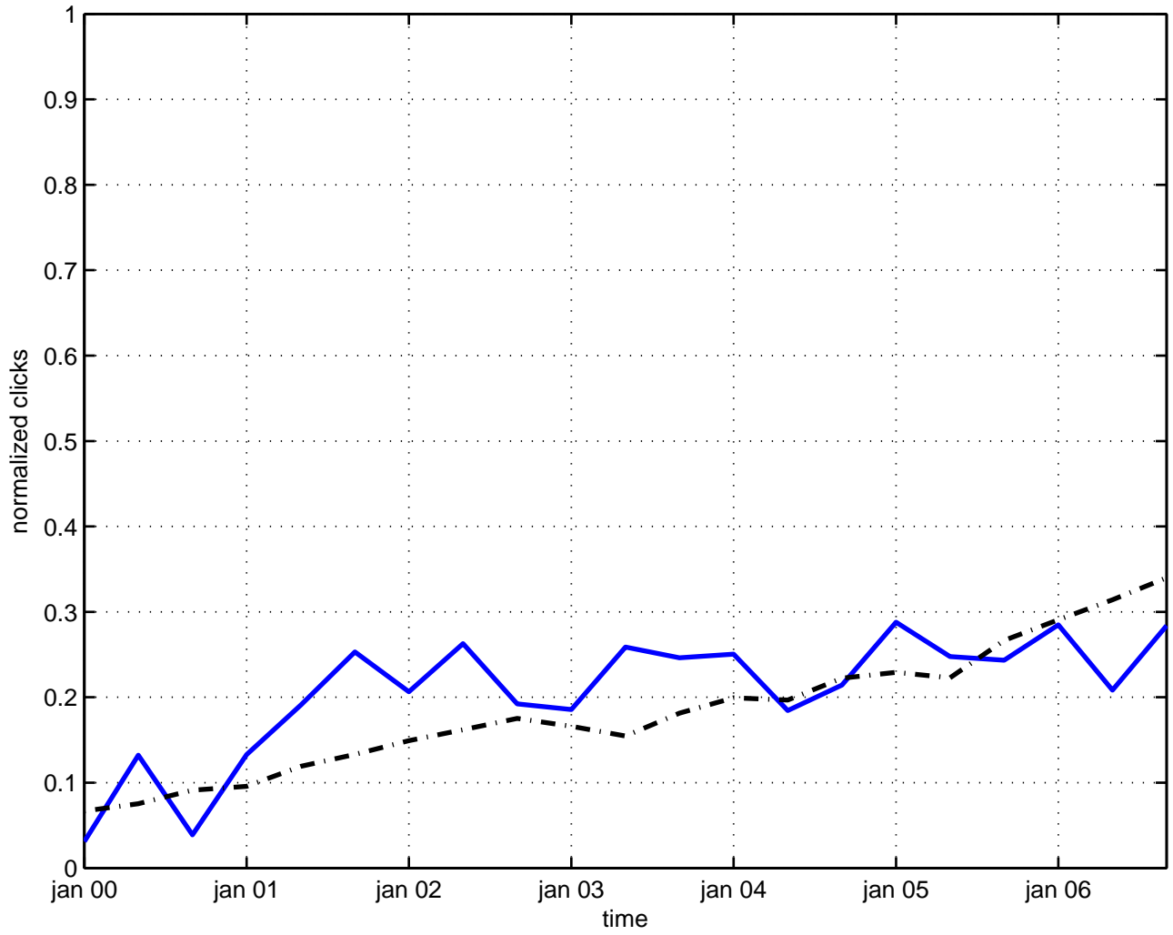
quantum group
