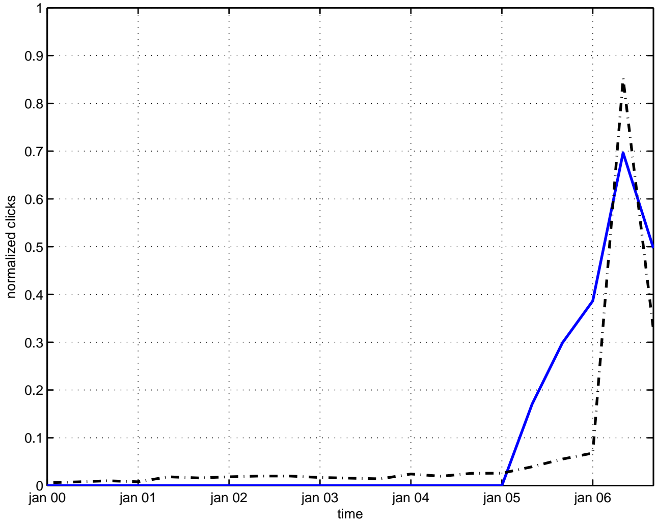
quantum correction
