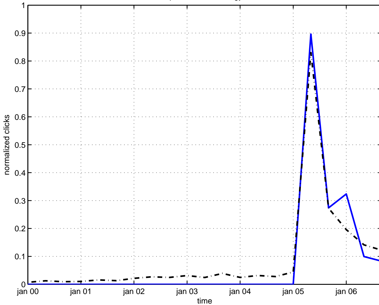
quantum cohomology
