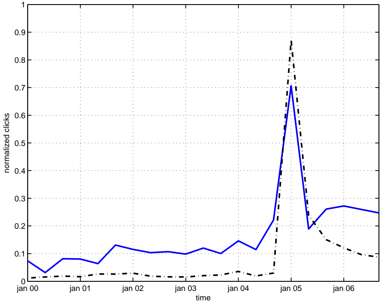
quantum chromodynamics
