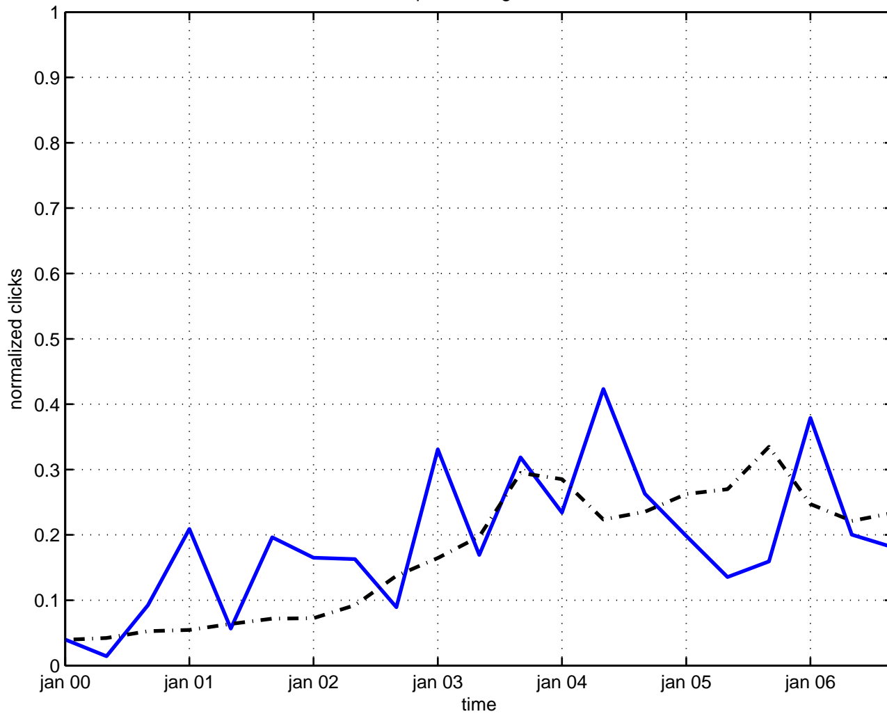
quantum algebra
