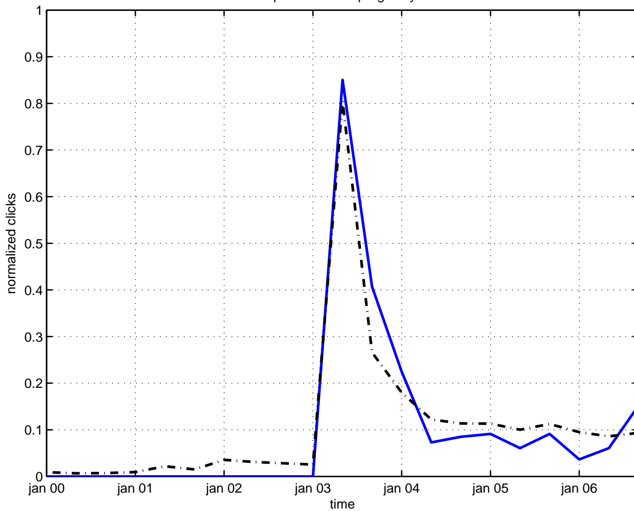
quantization supergravity
