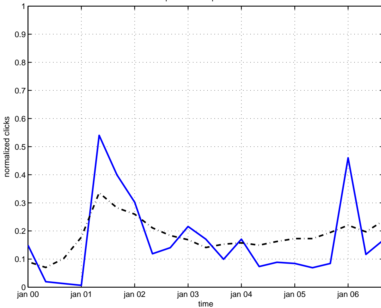
quantization space-time
