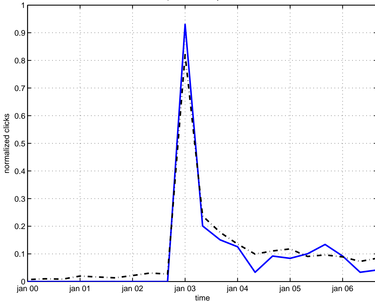
quantization skyrmion
