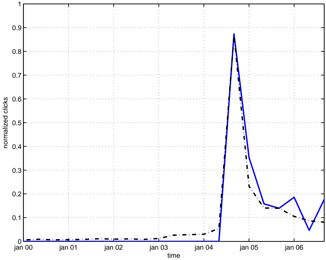
quantization perturbation
