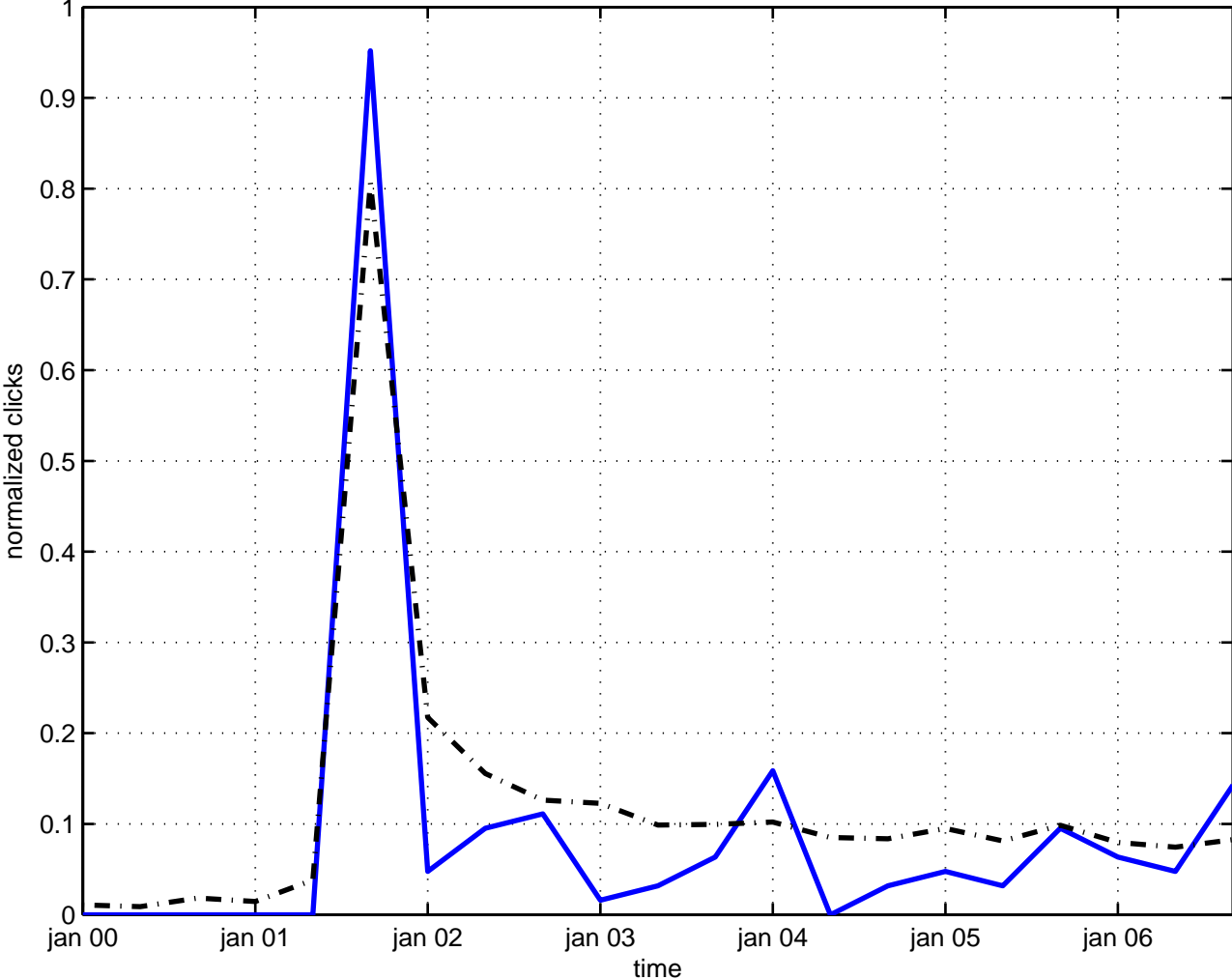
quantization path integral
