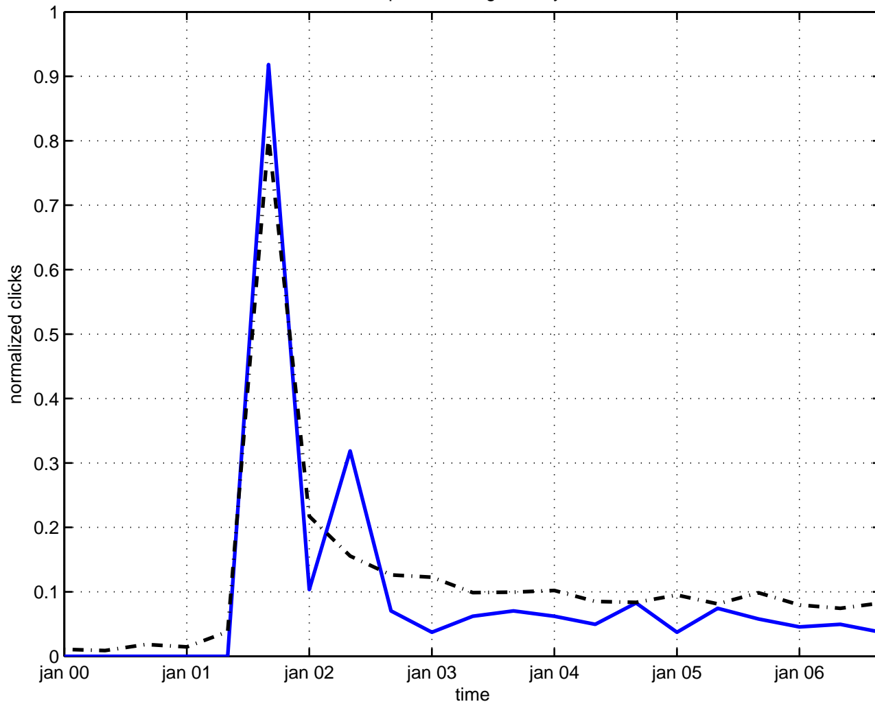
quantization geometry
