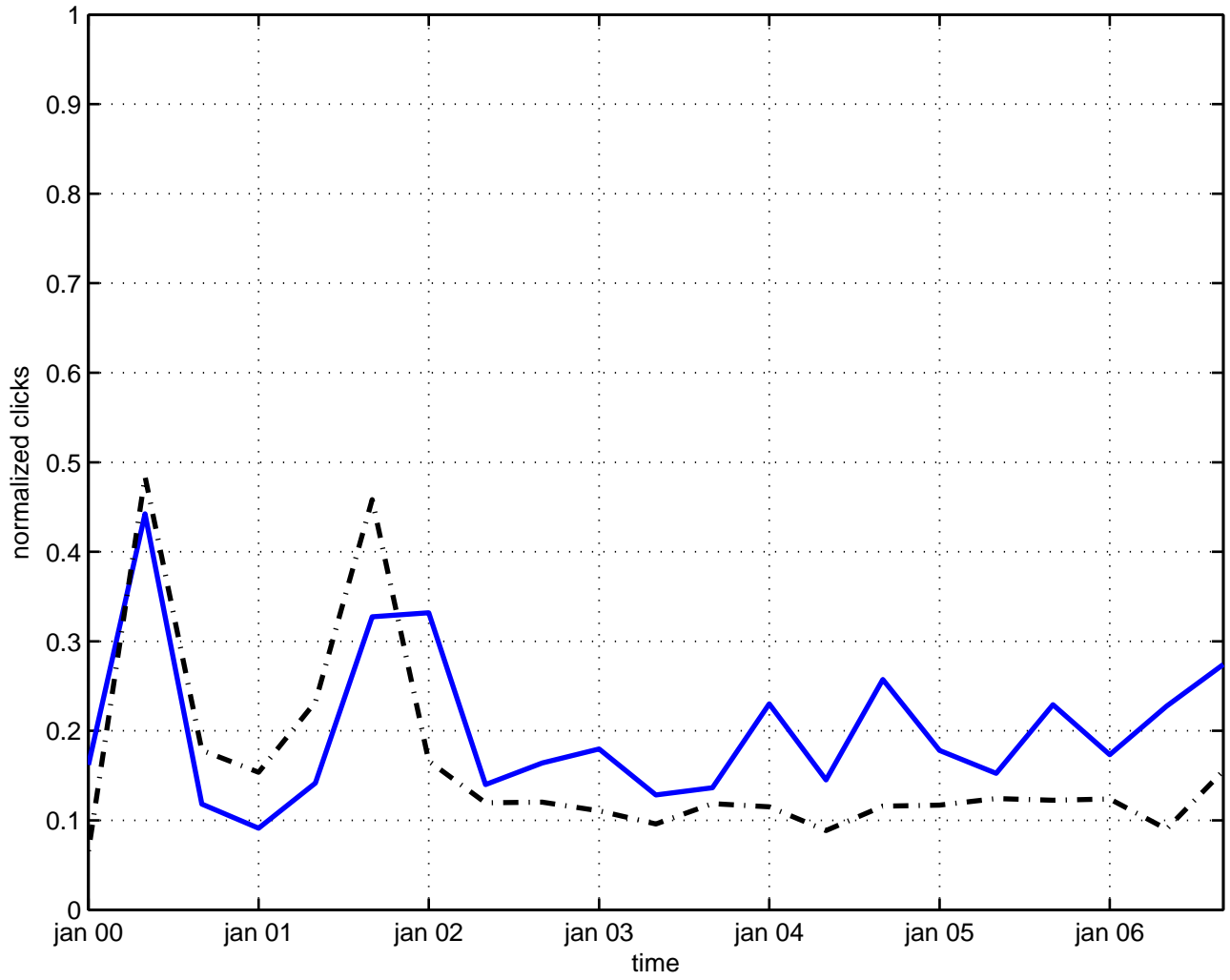
quantization flux
