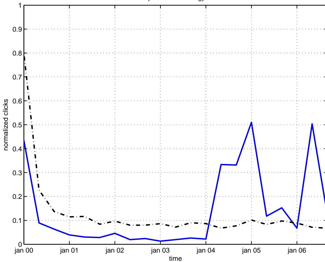
quantization energy
