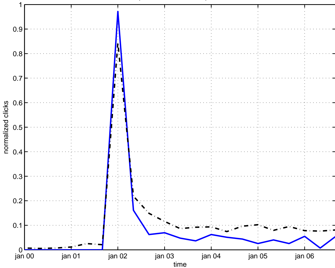
quantization diffeomorphism
