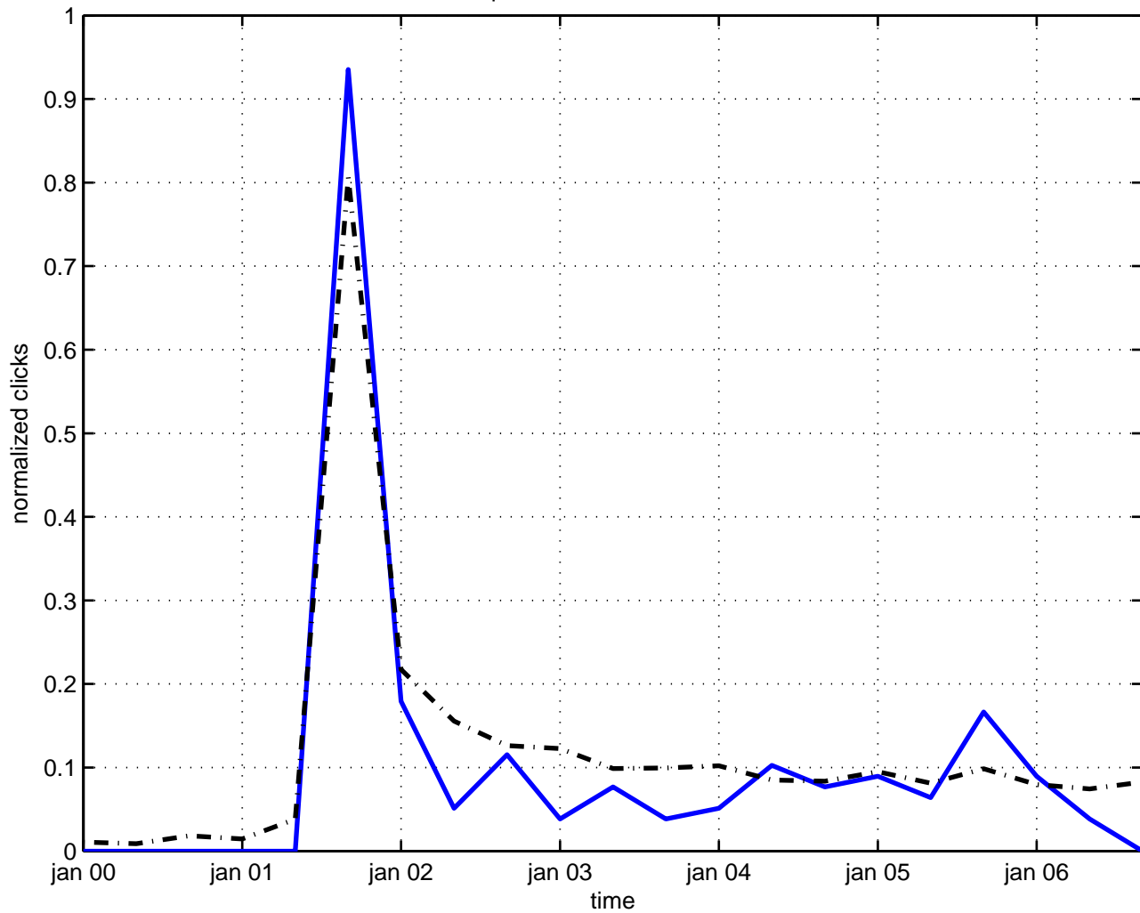
quantization deformation
