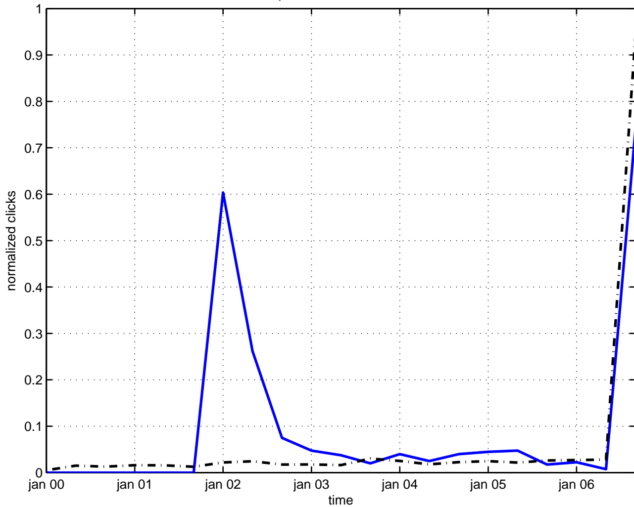
quantization black hole
