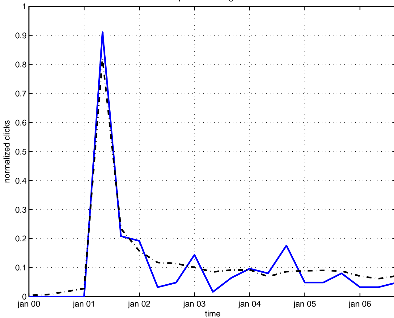
quantization algebra
