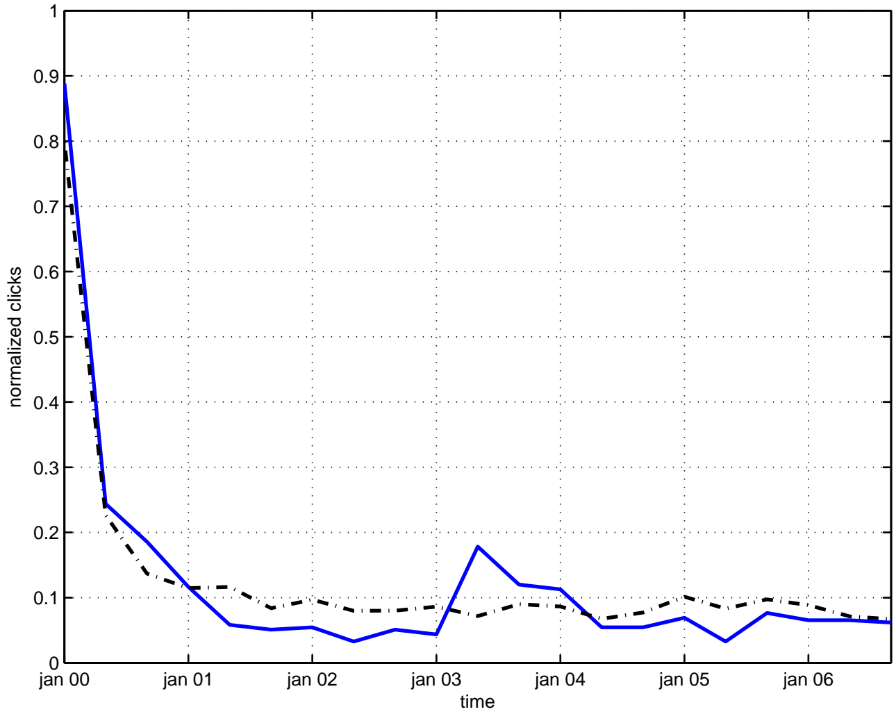
propagator pi
