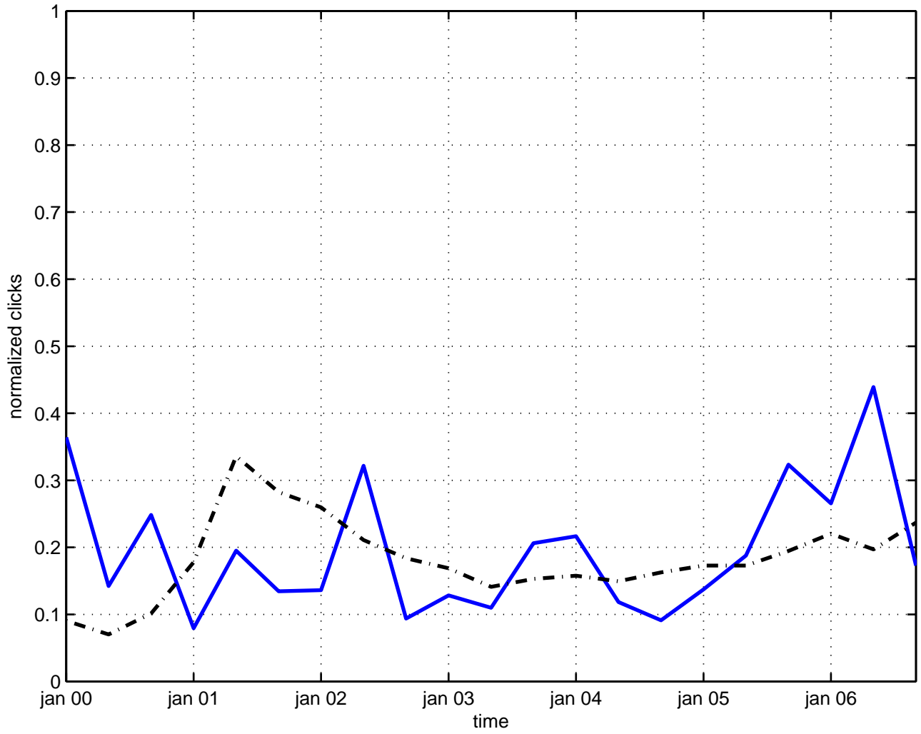
propagator photon
