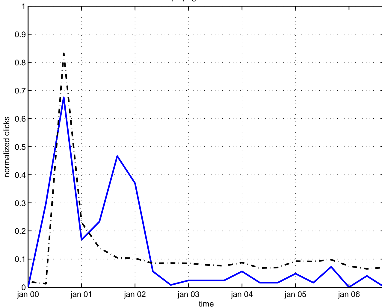
propagator neutrino
