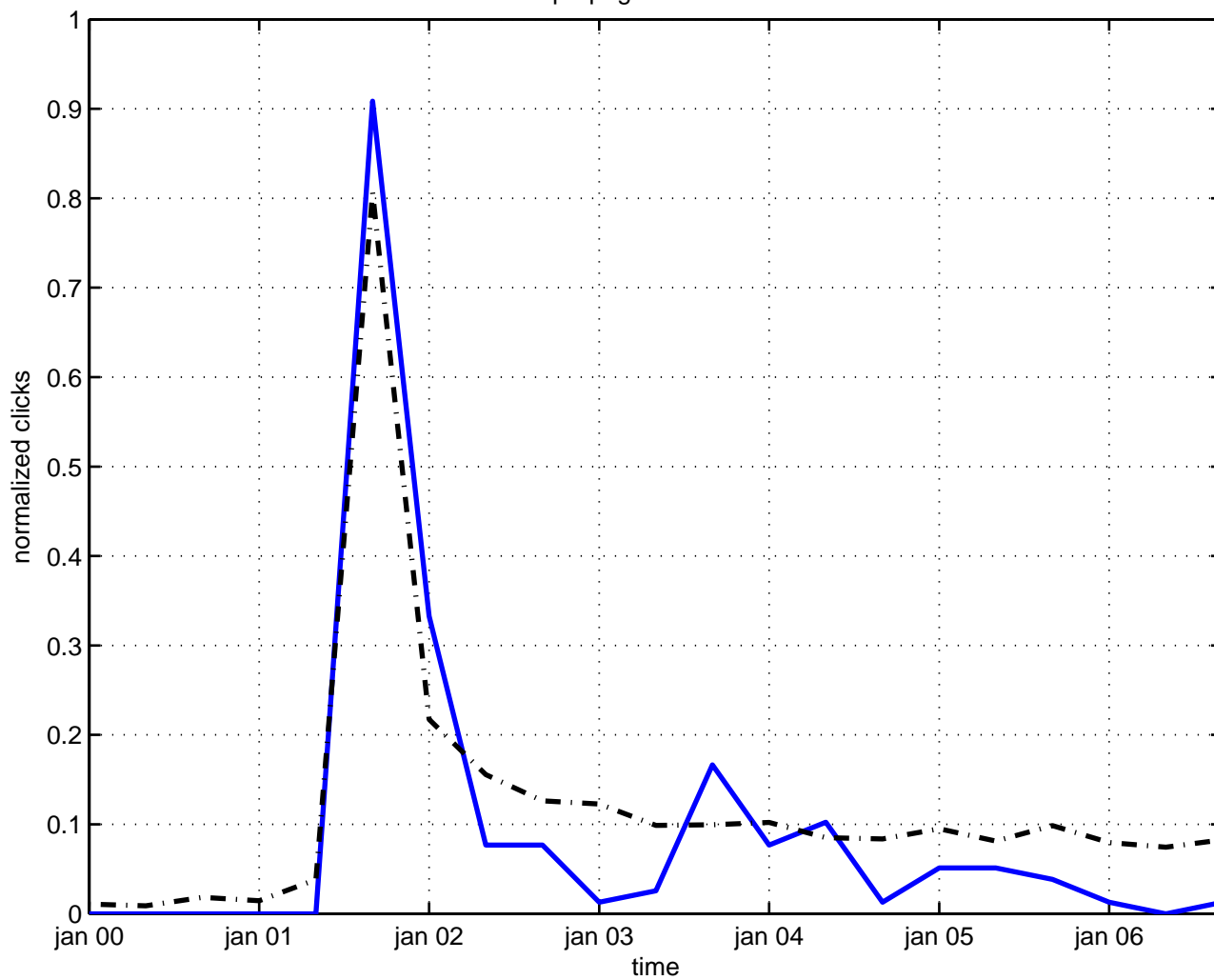
propagator meson
