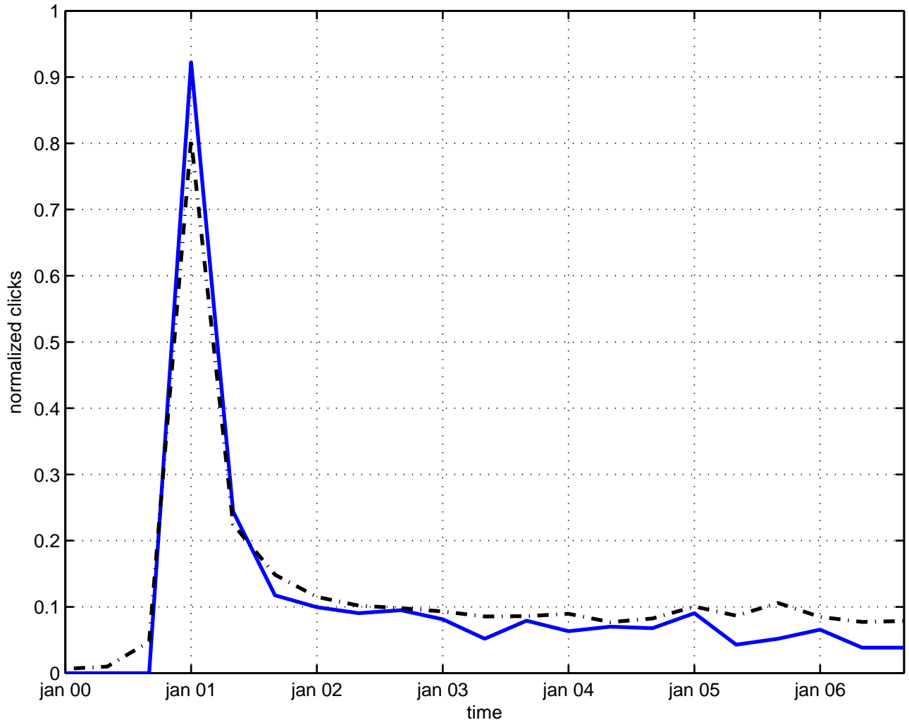
production tachyon
