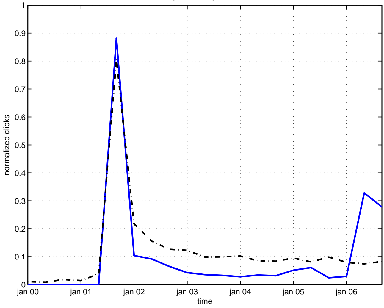
production photon
