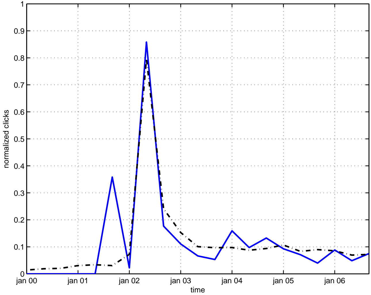
production intermediate boson
