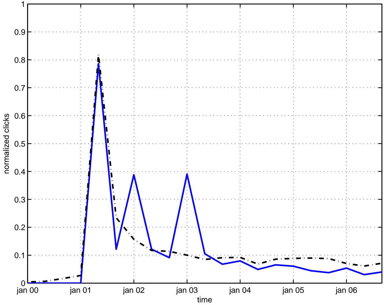
production domain wall
