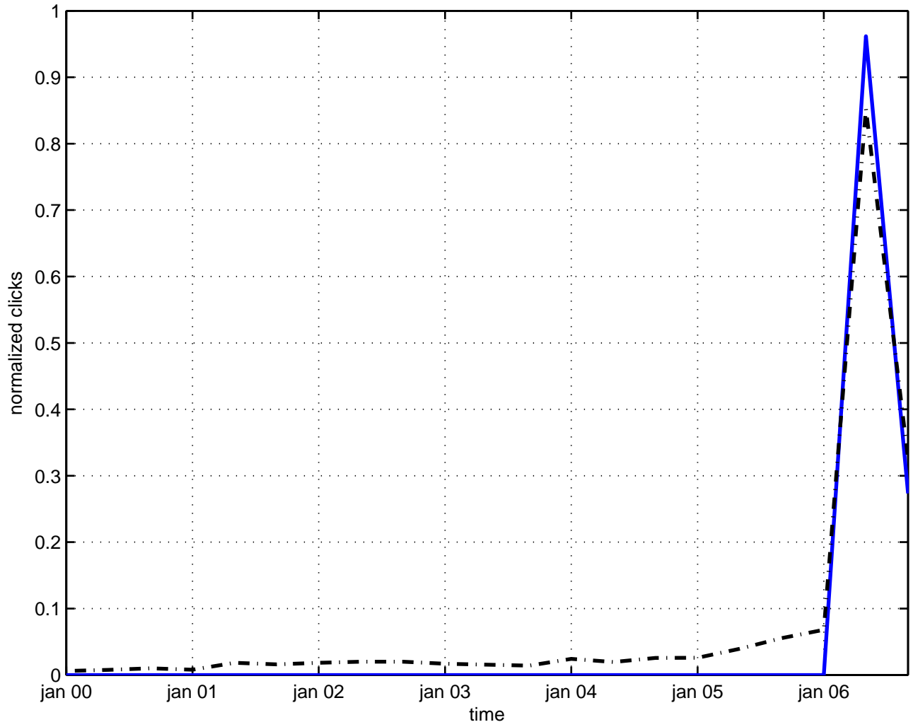
power spectrum oscillation
