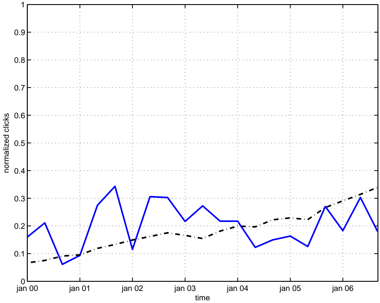
potts model
